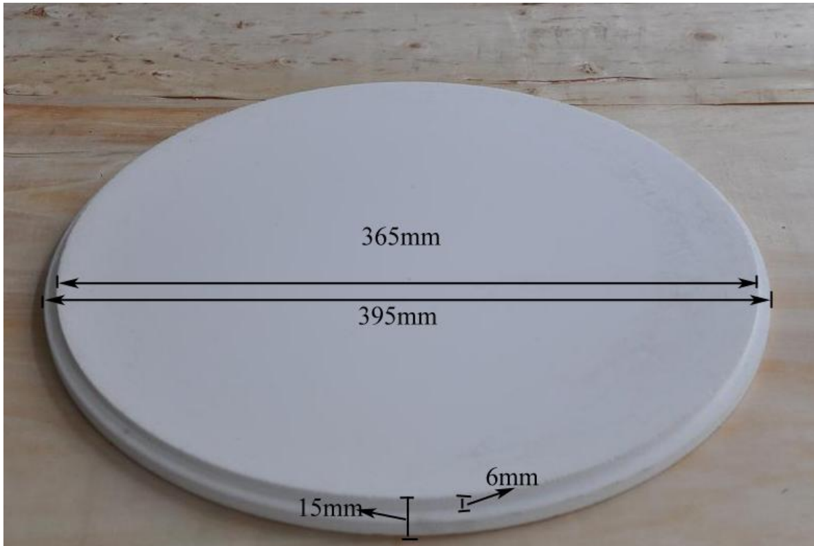
Fluid plate for powder hopper.
